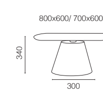
ROLL COFFEE TABLE 224
