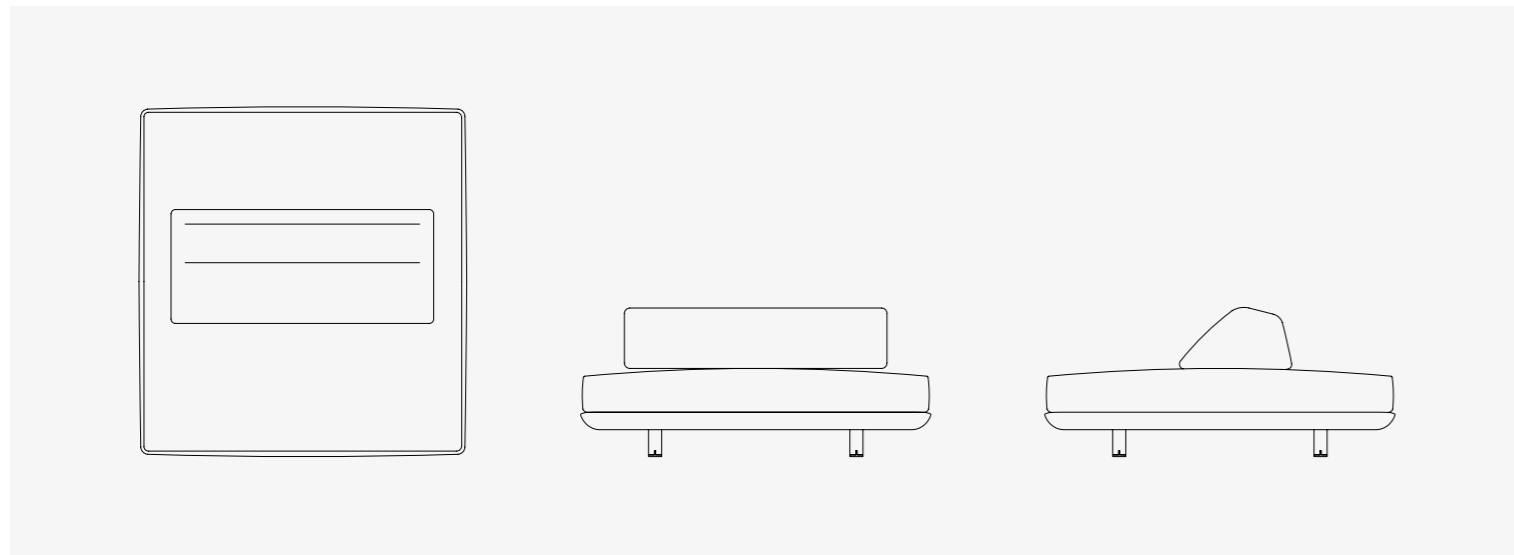
Island with standard fixed backrest (L & R) - 160×150×68 cm
