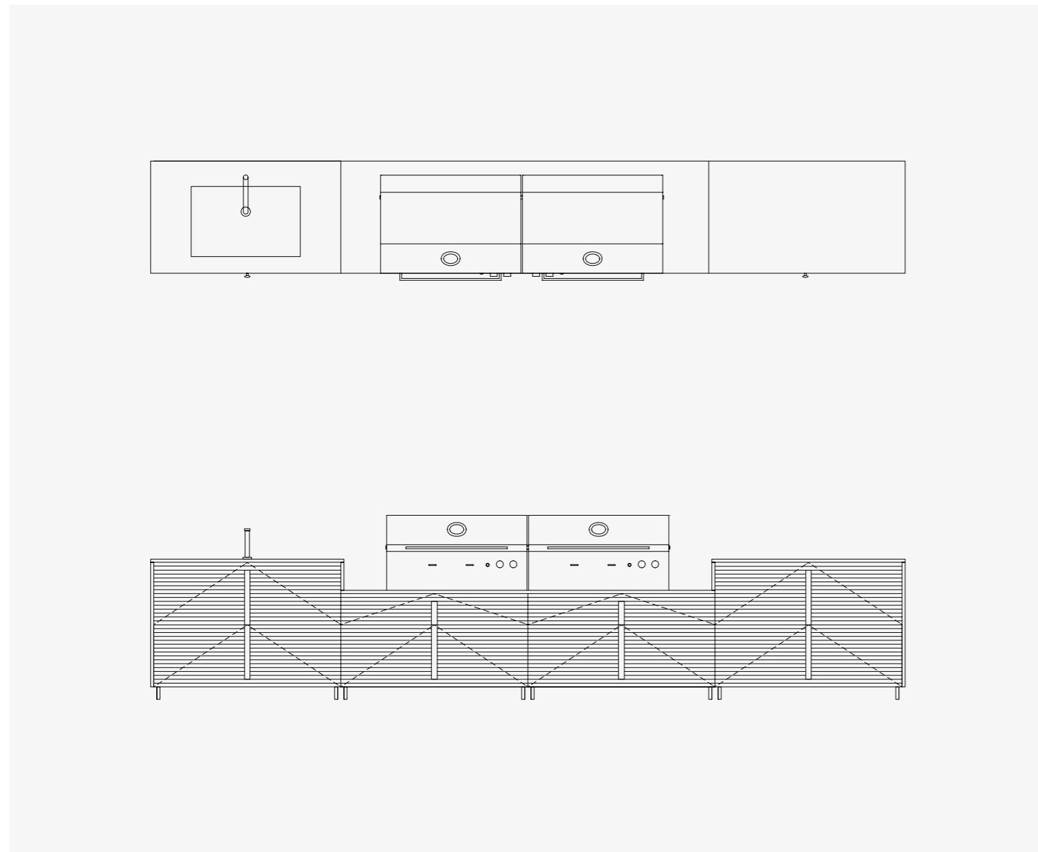
Amalfi Kitchen composition 04 - 484x72 cm
