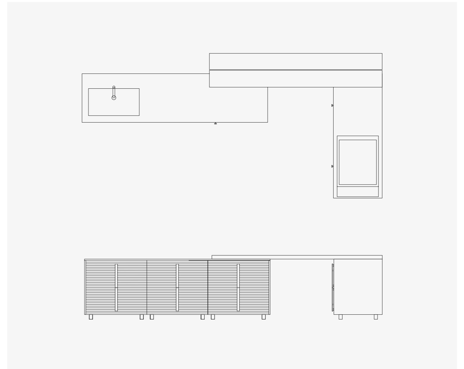
Amalfi Kitchen composition 05 - 443x214 cm
