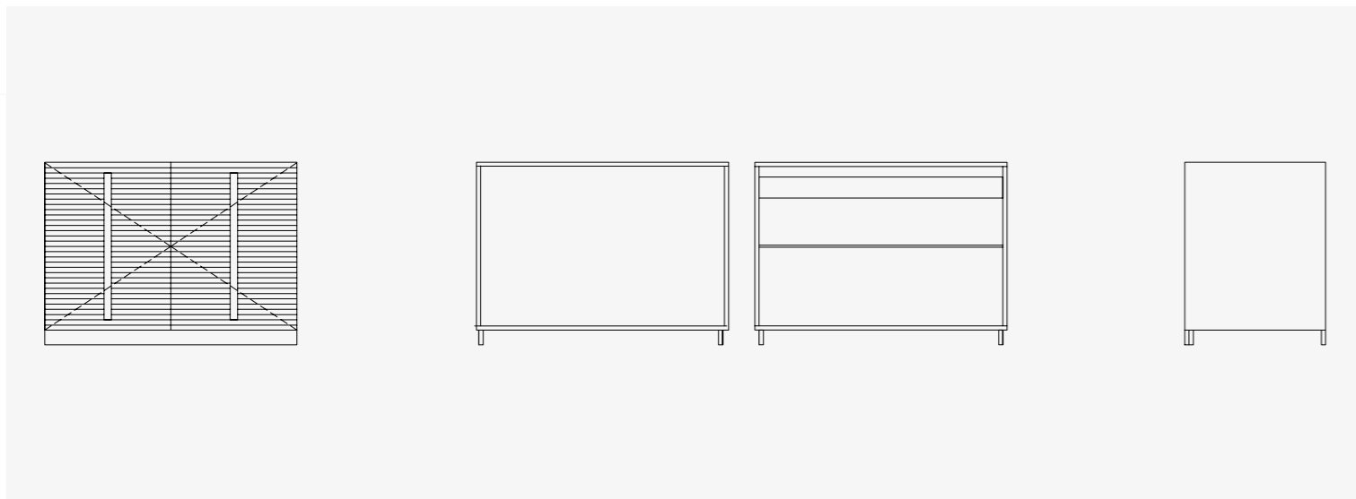
Storage bases 120 - Pull-out drawers - 120×70×87 cm
