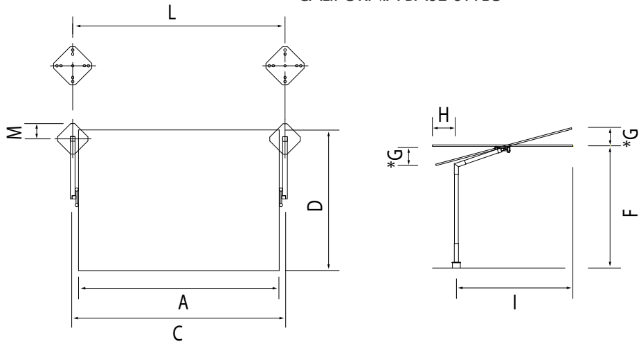
CALIFORNIA BASE STYLO
