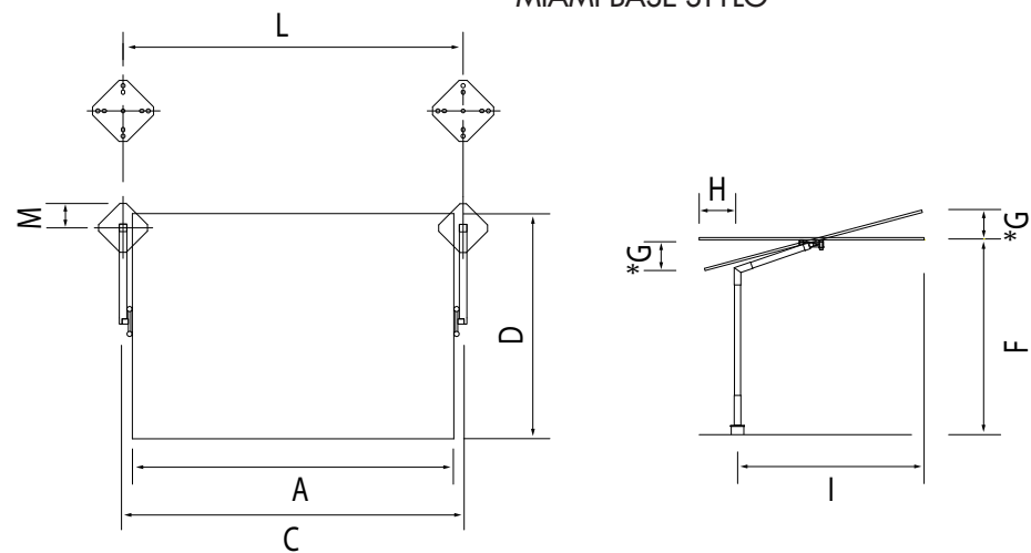
MIAMI BASE STYLO
