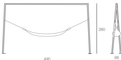
B132SE structure
