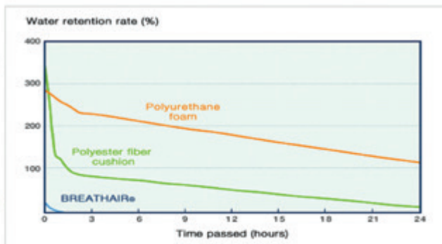
Toyobo Skin Model Method Heated plate: 37°C Amount of perspiration generated: 120g/m²-h Measurement environment: 20°C 60% RH
