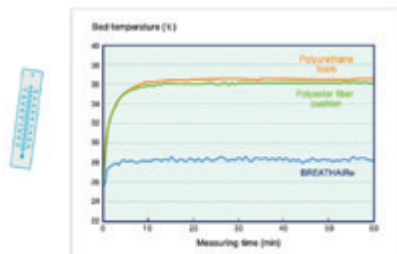
Toyobo Skin Model Method Heated plate: 37°C Amount of perspiration generated: 120g/m²-h Measurement environment: 20°C 60% RH
