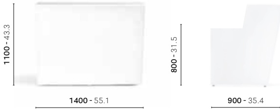
OBL/A soft Padded version of linear module
