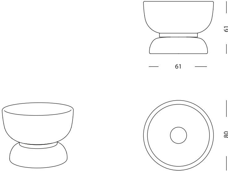
- 67440 Vase holder ø 80 x h 61
