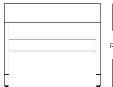
- 72224 Square armchair 85 x 82 x h' 40 x h 71 cm
