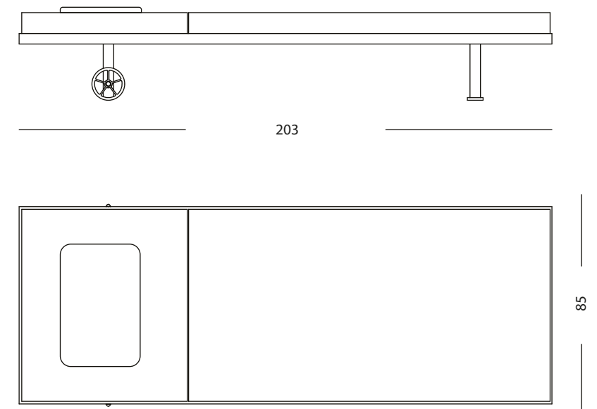
- 71882 Sunbed 203 x 85 x h 40 cm
