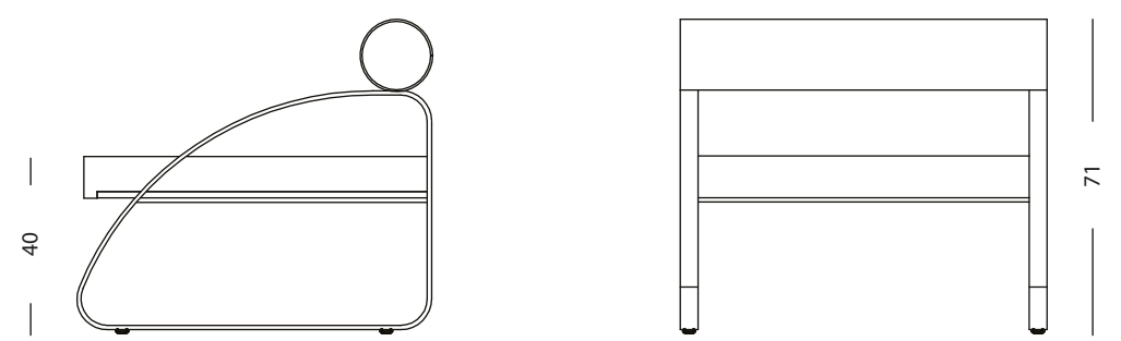
- 72222 Round armchair 83 x 82 x h' 40 x h 71 cm
